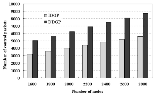
Fig. 16. Comparison of control packet overhead between IDGP and DDGP in 1000\text{ m} \times 500\text{ m} network area.
